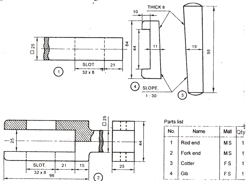
Fig. 1 COTTER JOINT WITH A GIB
