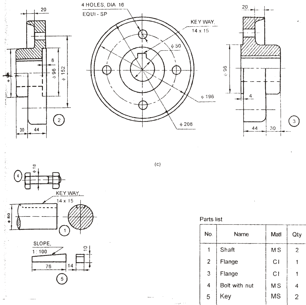
Fig.2 PROTECTED FLANGED COUPLING
